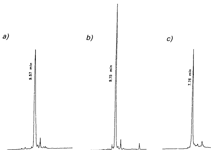
Fig. 1. Reversed-phase HPLC of a) crude p60 wrc -(523–531)-nonapeptide, obtained with O 4 - Bu t -protected Tyr, b) crude p60 wrc -(523–531)-nonapeptide, obtained with side-chain-unprotected Tyr, and c) crude O 4,527 -phospho-p60 wrc -(523–531)-nonapeptide (3) prepared by global phosphorylation. Conditions: 0–100% MeCN in 0.05% CF 3 COOH, 30 min, λ = 230 nm.
